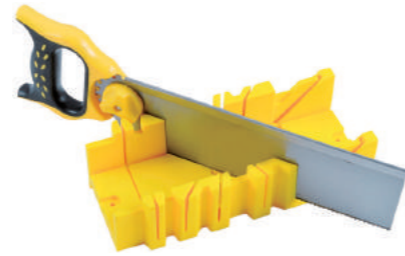
HK5007 ▶ Back Saw With Miter Box Material:High Carbon Steel Blade, PP+TPR Handle,Miter Box PP
