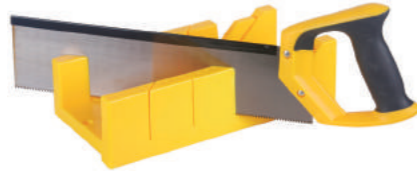
HK5006 ▶ Back Saw With Miter Box Material:High Carbon Steel Blade, PP+TPR Handle,Miter Box PP
